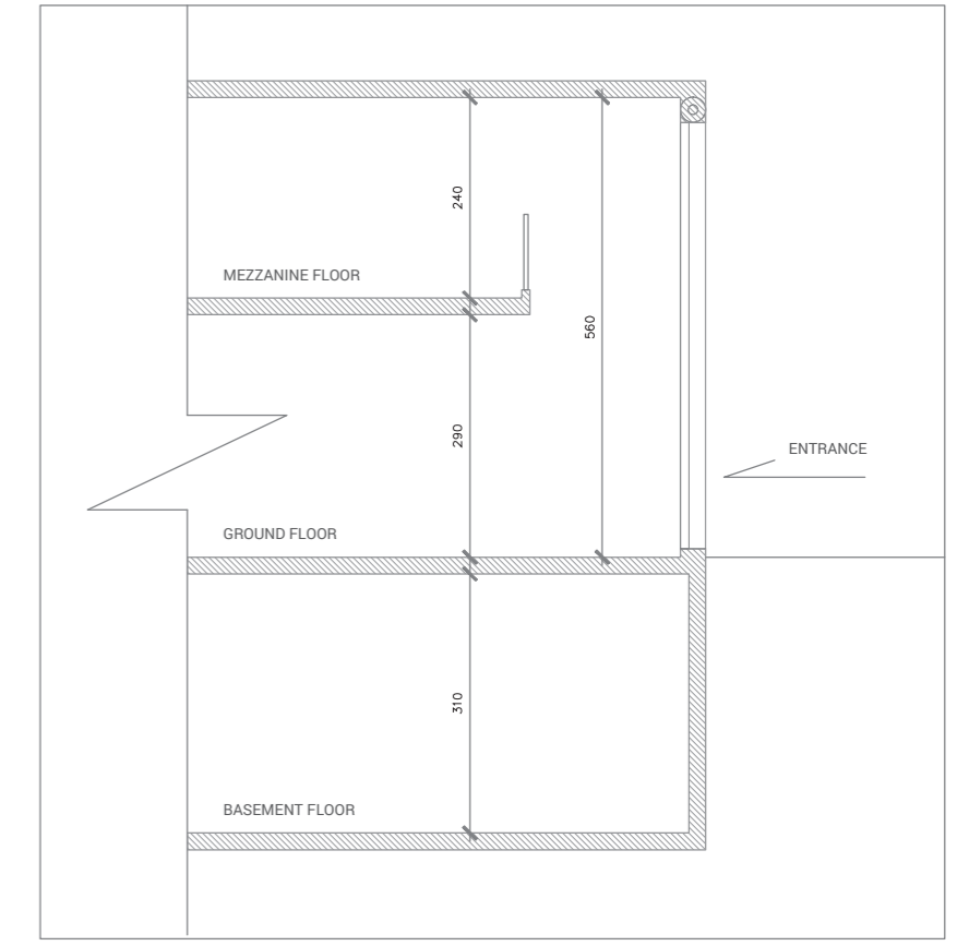
GROUND FLOOR / MEZZANINE SHOP SECTION
